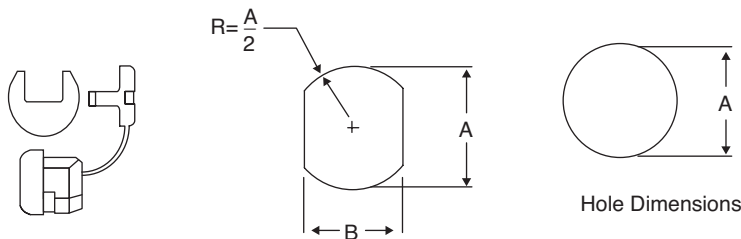
Bushing Dimensions
